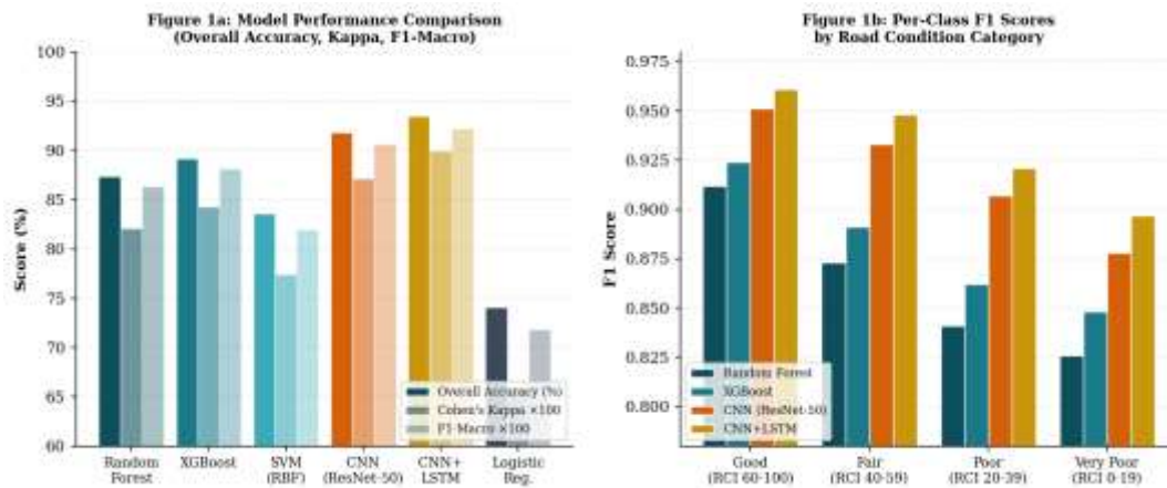
Figure 1: Model performance comparison. Left: Overall Accuracy, Kappa (100), and F1-Macro (100) for all six models. Right: Per-class F1 scores for the four best-performing models across the four road condition categories.
