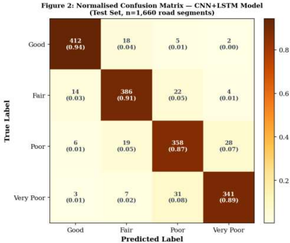
Figure 2: Normalised confusion matrix for the CNN+LSTM model on the held-out test set (n=1,660 road segments). Cell values show absolute counts (top) and normalised proportions (bottom). Colour intensity indicates proportional accuracy.
