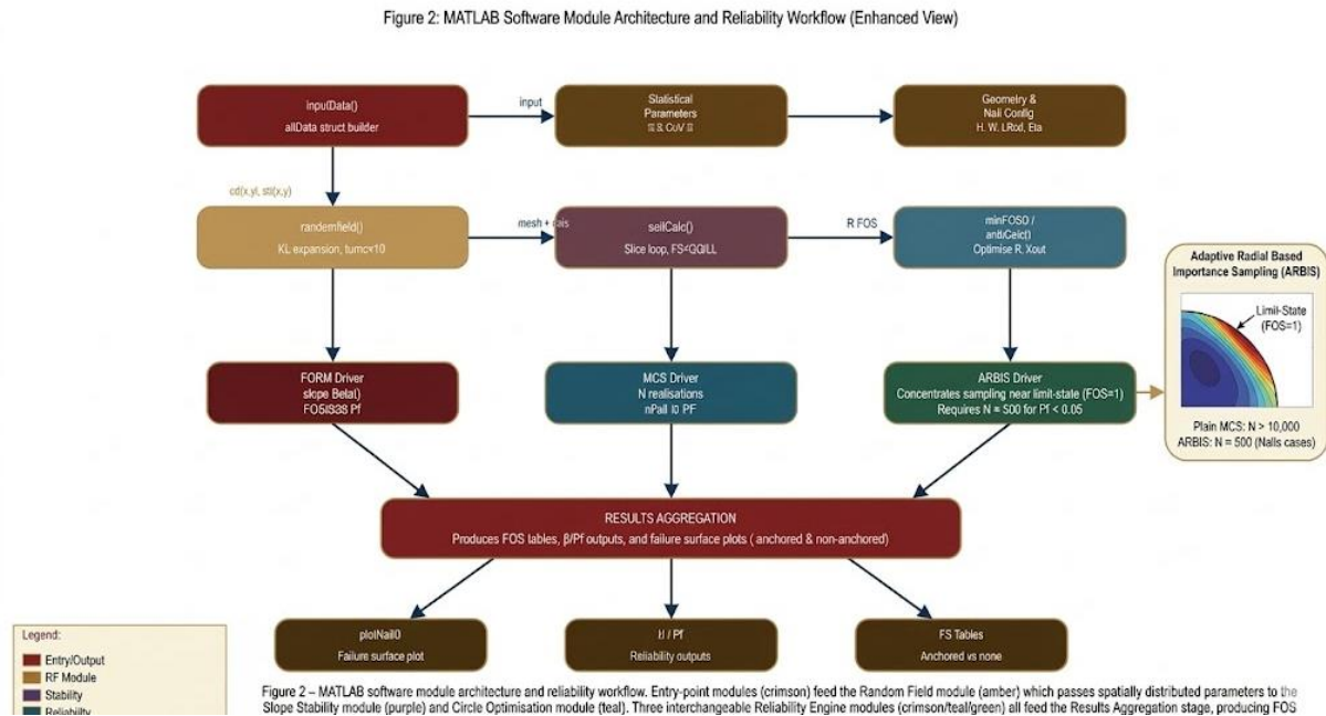
Figure — Figure 2 – MATLAB software module architecture and reliability workflow. Entry-point modules (crimson) feed the Random Field module (amber) which passes spatially distributed parameters to the Slope Stability module (purple) and Circle Optimisation module (teal). Three interchangeable Reliability Engine modules (crimson/teal/green) all feed the Results Aggregation stage, producing FOS tables, \beta/P_f outputs, and failure surface plots.
