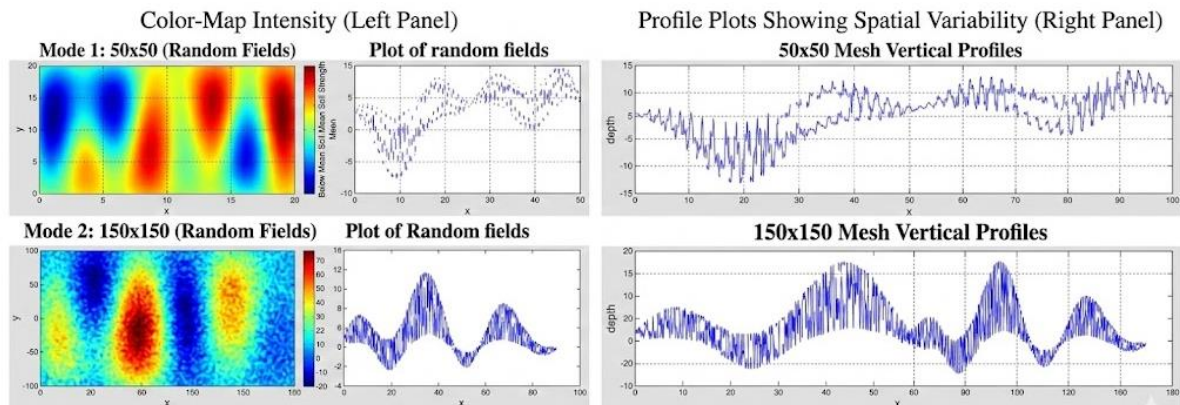
Figure — Example random field output maps from MATLAB. Top row: 50 \times 50 mesh (coarse realisation). Bottom row: 150 \times 150 mesh (fine realisation). Left panels: colour-map intensity (blue = below mean, red = above mean). Right panels: profile plots showing spatial variability across the mesh. Source: Dissertation Figure 4.2.
