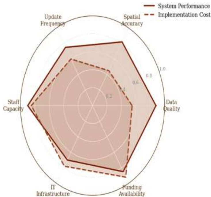
Figure 7. Sensitivity Analysis Radar Chart — Influence of Six Enabling Factors on BIM-GIS System Performance (crimson) and Implementation Cost (sienna). Based on expert elicitation ( n = 23 ), normalised to maximum = 1.0.
