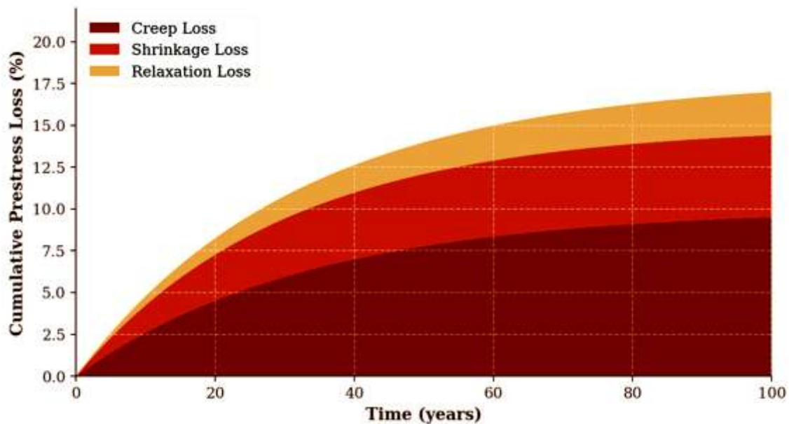
Figure 3. Time-Dependent Prestress Loss Components in the Post-Tensioned Box Girder (Baseline Case: f_{ck} = 32 \text{ MPa} , \text{RH} = 60\% , T = 30^\circ\text{C} , Initial Prestress = 75% GUTS).
