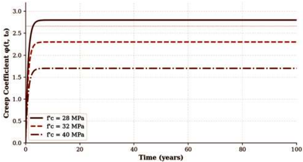
Figure 1. Creep Coefficient Development with Time for Varying Concrete Grades (CEB-FIP MC2010; RH = 60%, T = 30°C, h 0 = 182 mm, t 0 = 28 days).
