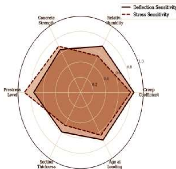
Figure 5. Sensitivity Analysis Radar Chart: Normalised Influence of Six Key Parameters on Long-Term Deflection (red) and Concrete Stress at Tendon Level (brown).
