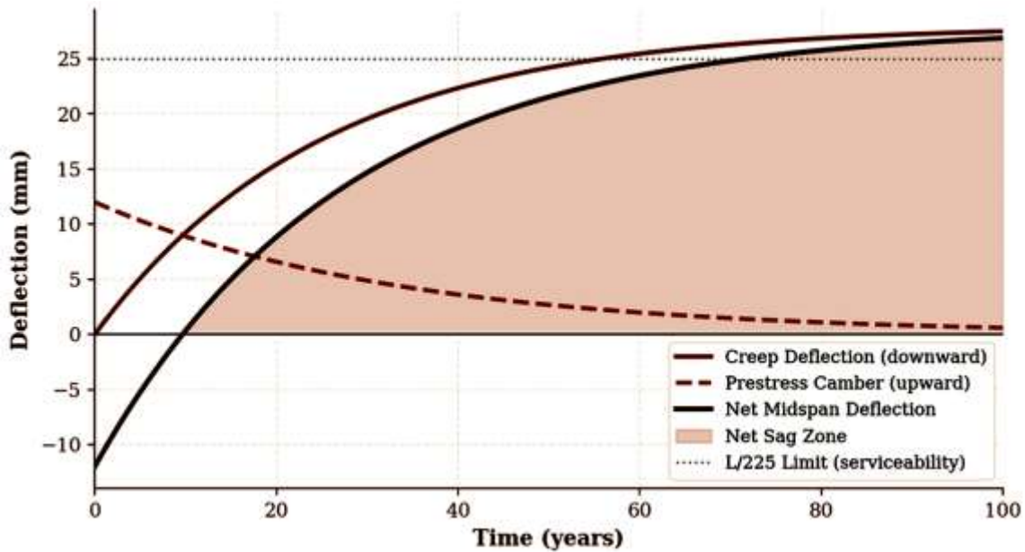
Figure 4. Midspan Deflection Evolution Over 100 Years: Creep Deflection vs. Prestress Camber and Net Response (Baseline Case, L = 40 m).
